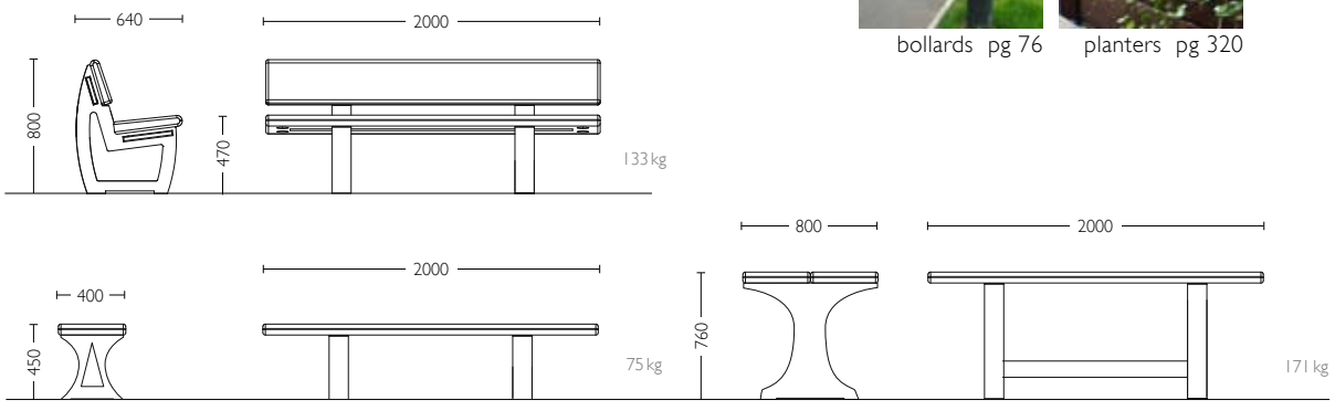
▲ ABERDEEN BENCH & TABLE brown recycled plastic
