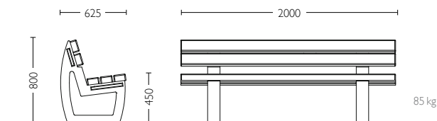
▲ PERTH SEAT, BENCH & TABLE brown recycled plastic standards brown recycled plastic slats
