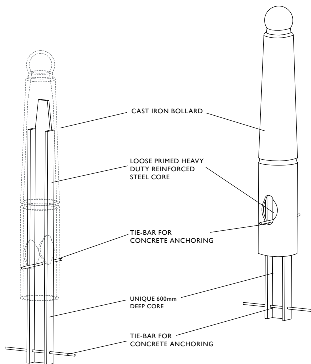
▲ TYPICAL CAST IRON SECURITY BOLLARD CONSTRUCTION GUNNER SECURITY shown here
